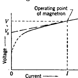
FIG. A-41.—Magnetron voltage-current characteristic under pulse conditions.
